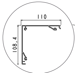
Perfil cofre Cassette profile
