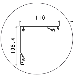
Perfil cofre Cassette profile
