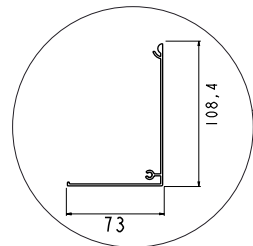
Perfil frontal cofre Cassette front profile
